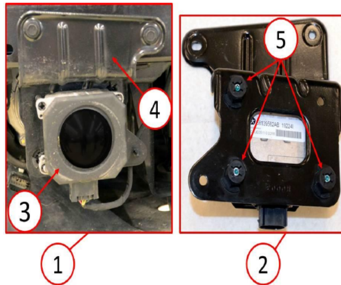
Fig. 1 Adaptive Cruise Control Sensor
